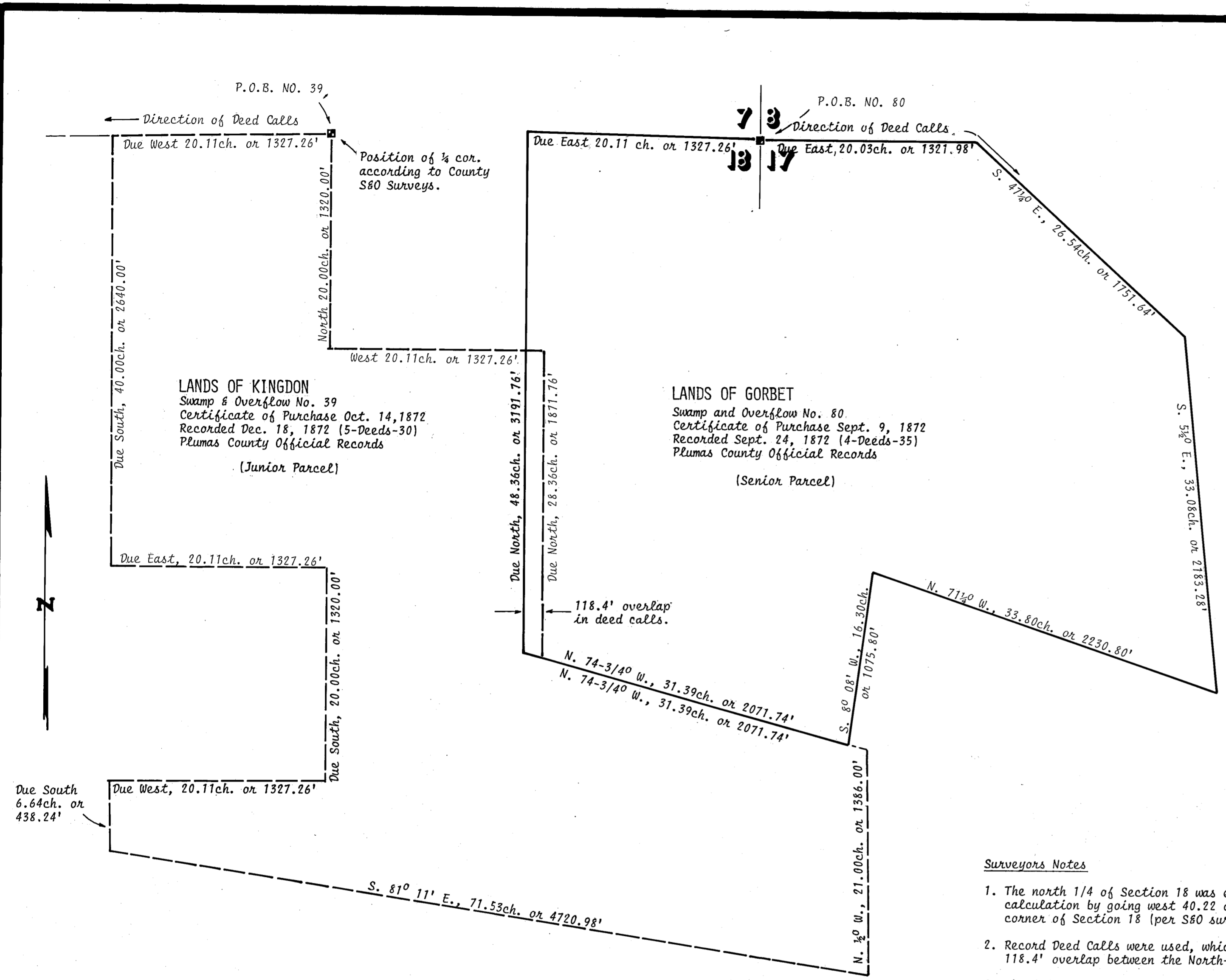
FIGURE 1. A PLOT OF DEED CALLS FROM SWAMP AND OVERFLOW SURVEYS NO. 39 AND 80 SHOWING AN OVERLAP ALONG ADJOINING BOUNDARIES.
