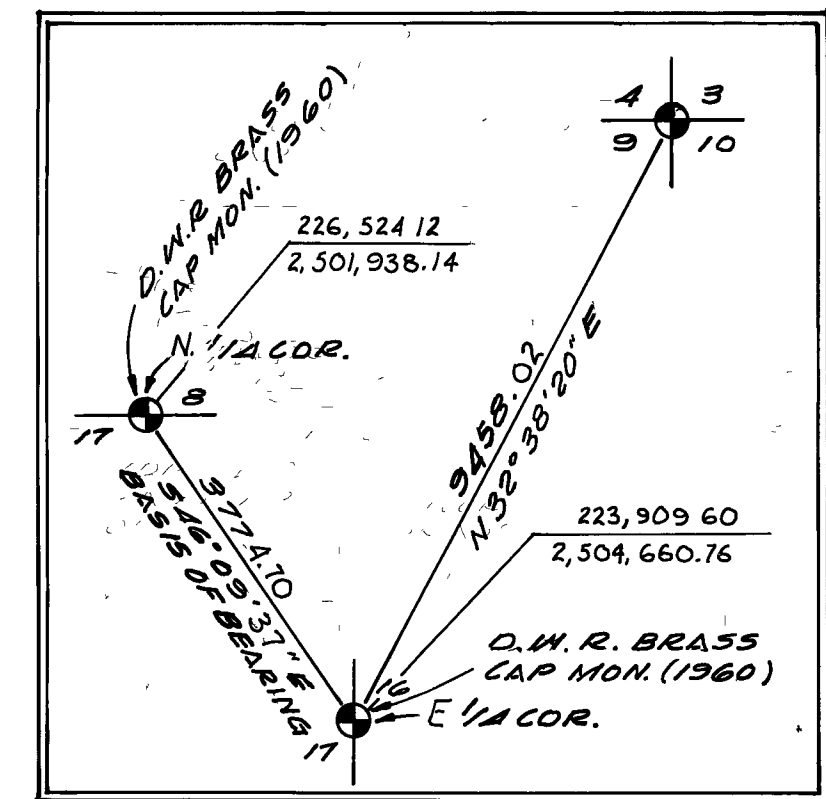
CONTROL SCHEMATIC NOT TO SCALE
