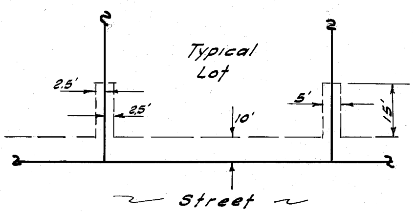
UTILITY EASEMENT DETAIL NO SCALE
